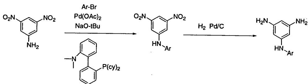
Scheme II-B
